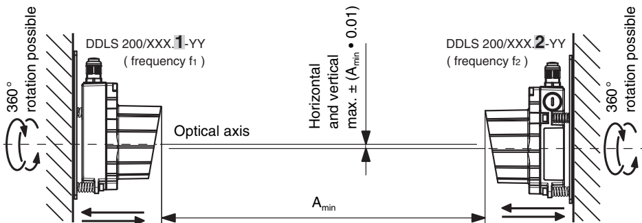
Figure 4.1: Mounting the devices
