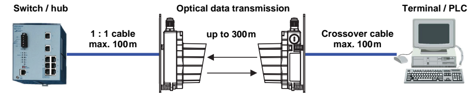
Figure 10.4: Network expansion
