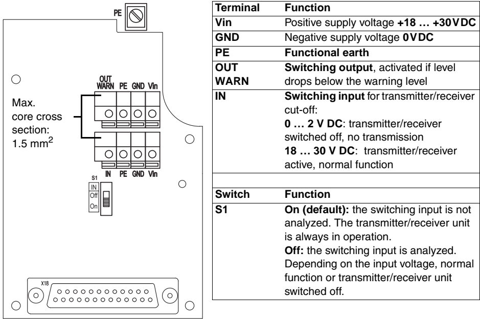
Figure 4.5: Positions of the general, non-bus-specific terminals and switches
