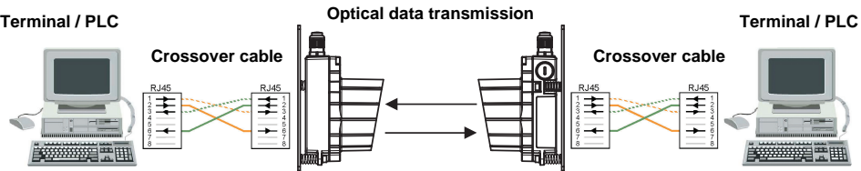
Figure 10.7:DDLS 200 between terminal/PLC and terminal/PLC
