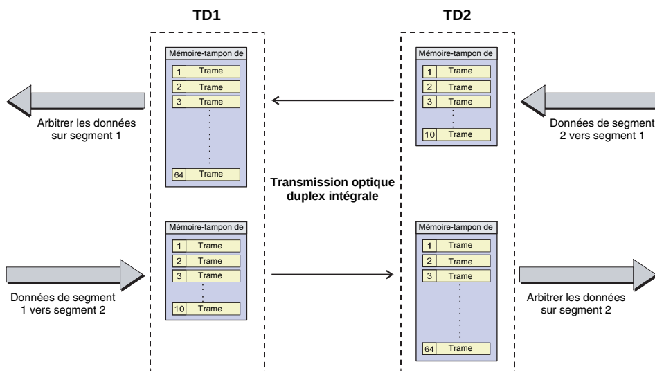
Figure 9.13: Division de segment
