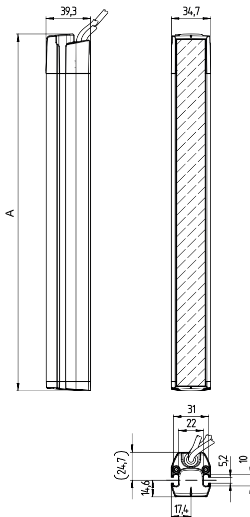
Fig. 12.1: Dimensions of transmitter and receiver
