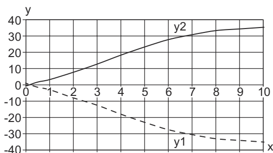
Typ. response behavior (TKS100x100)
