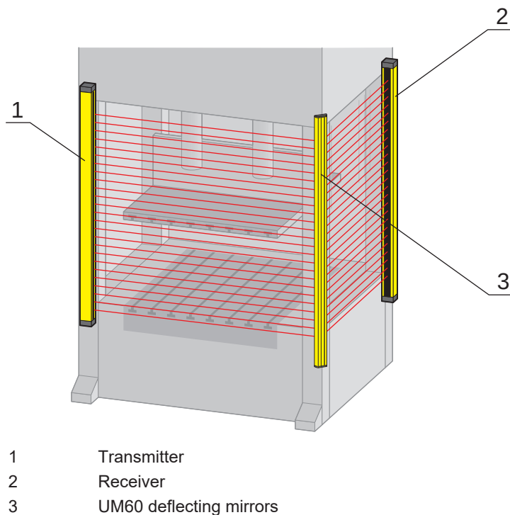
Fig. 6.11: Arrangement with deflecting mirror for 2-side guarding of a point of operation
