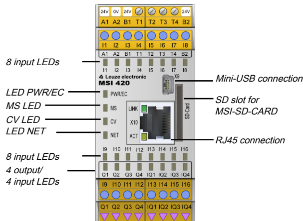
Fig. 3.6: Display elements of a MSI 420-x module
