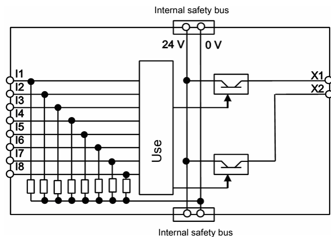
Fig. 3.10: Internal circuits of the MSI-EM-IO84 module: Safe inputs and test outputs
