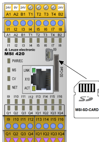
Fig. 3.1: Example of a minimum MSI 400 system setup with a MSI 430-01 controller module
