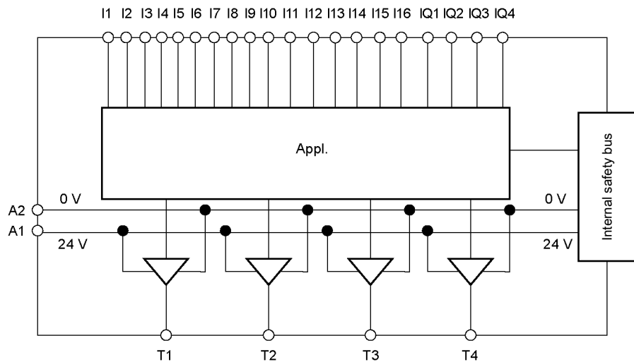
Fig. 3.7: Inputs and test pulses at an MSI 420-x module
