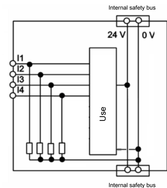
Fig. 3.16: Internal switching circuit of the MSI-EM-IO84NP module: non-secure inputs
