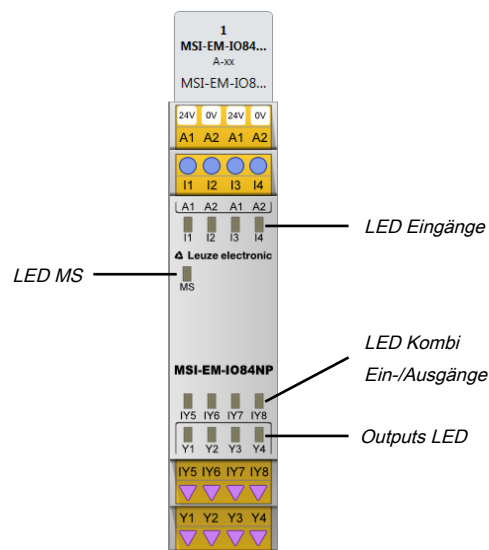
Fig. 3.15: Display elements of the MSI-EM-IO84NP module
