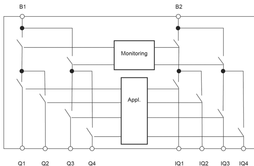
Fig. 3.8: Outputs at an MSI 420-x module
