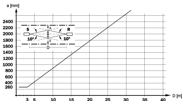
Fig. 4.3: Minimum distance "a" as a function of distance "D" for testable single-beam safety light barriers with 10° aperture angle
