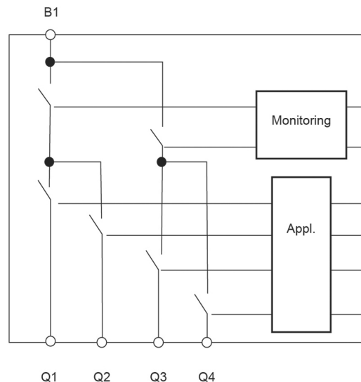
Fig. 3.5: Outputs at an MSI 410 module
