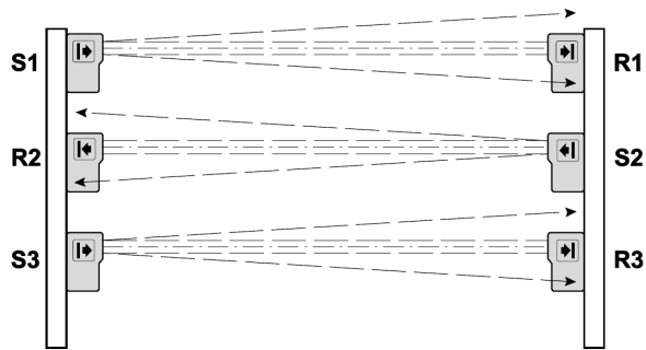
Fig. 4.4: Installation so as to prevent optical interaction
