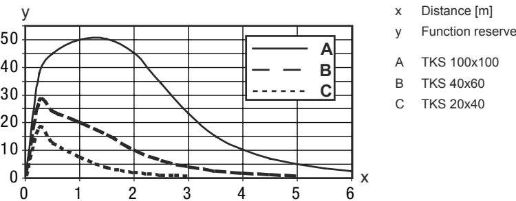
Typ. function reserve
