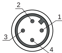
Fig. 5.1: Transmitter pin assignment
