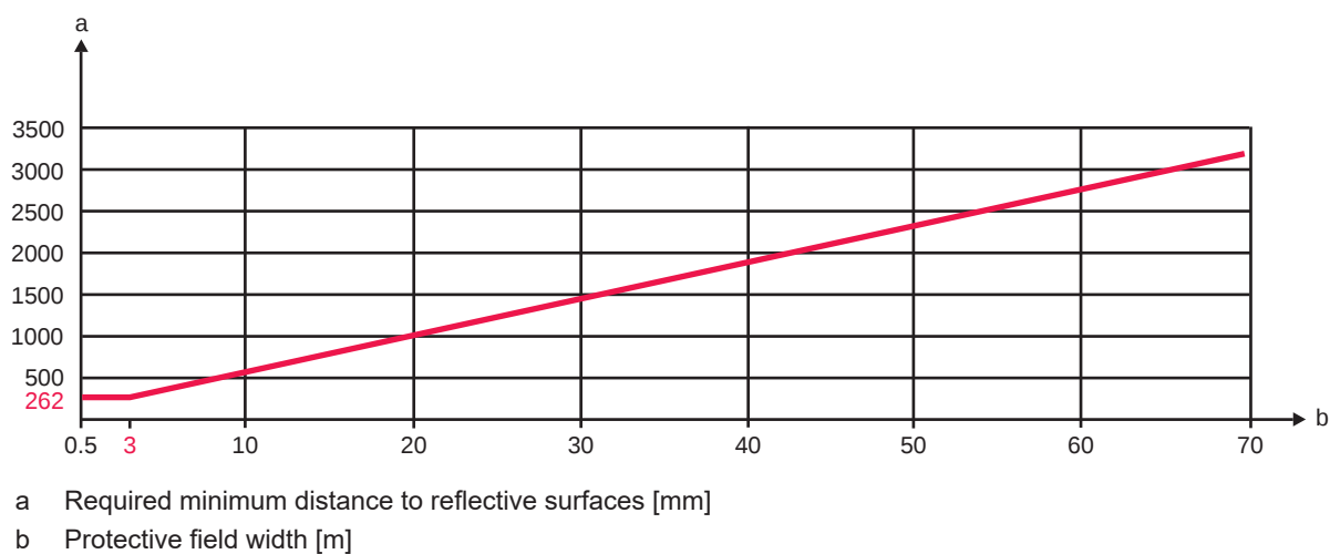
Fig. 4.4: Minimum distance to reflective surfaces as a function of the protective field width
