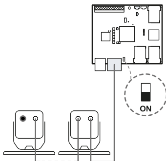
Chain with controller at the end of the chain and a sensor with termination connector
