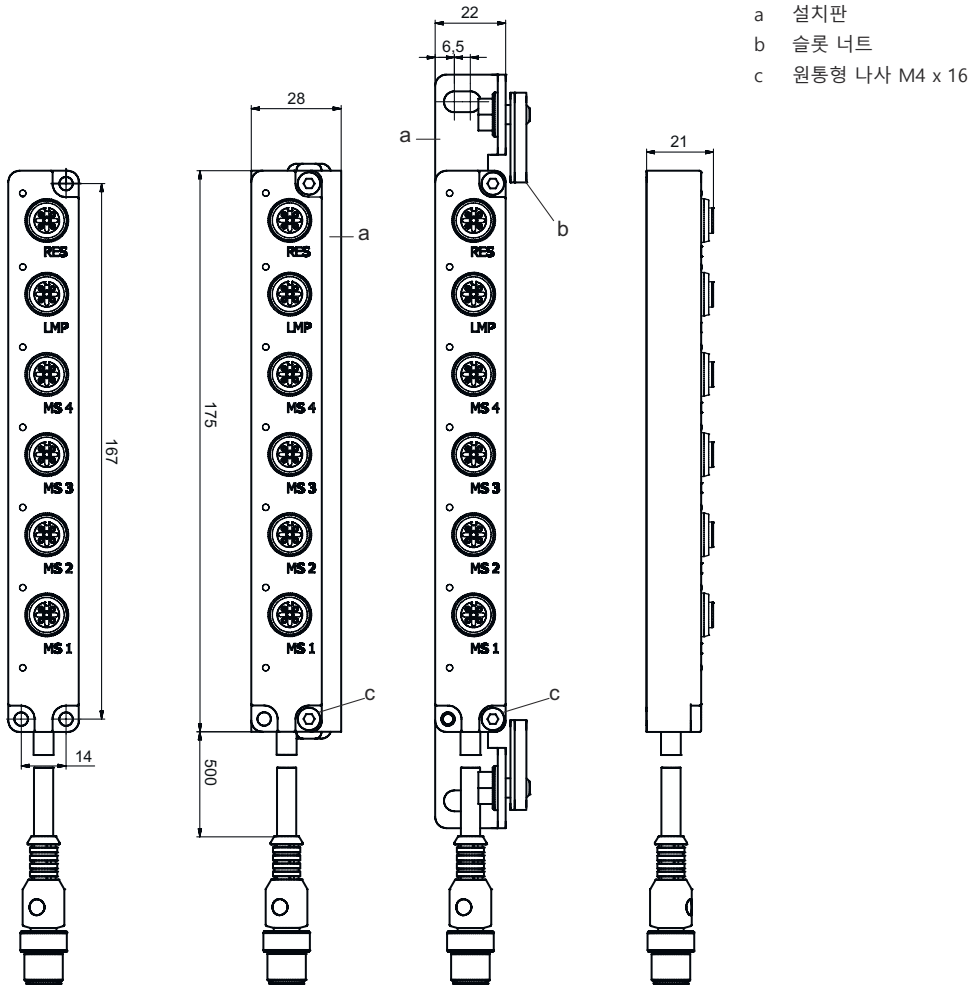
AC-SCM7U
