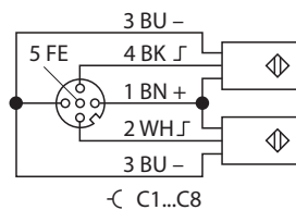
Fig. 6.3: Pin assignment MD 742-11-82X5-12 (C1...C8)
