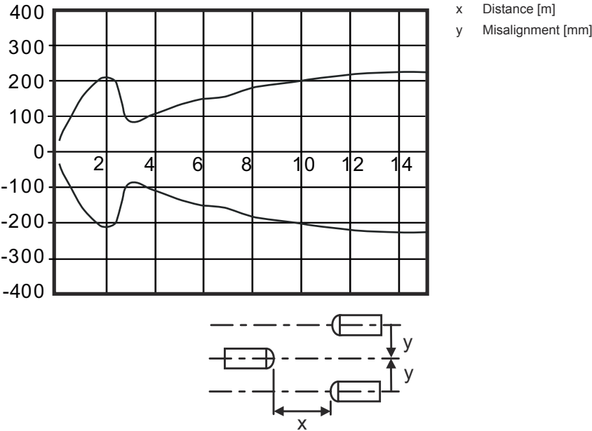
Typ. response behavior
