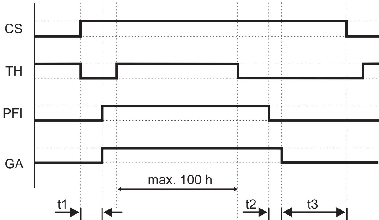
Fig. 4.11: SPG timeout extension
