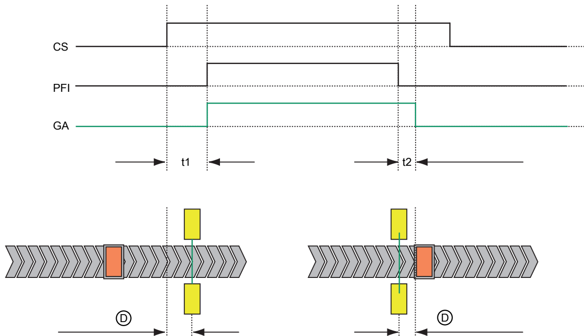
Fig. 4.2: SPG principle
