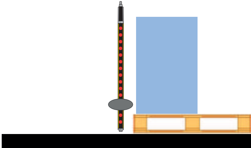
Fig. 4.3: Protective field violation with reduced resolution and object in the protective field
