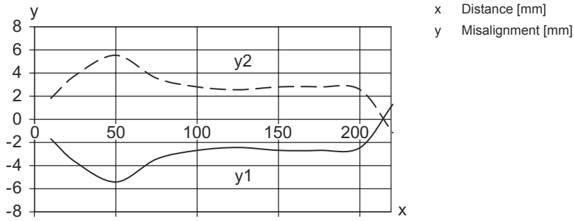
Typ. response behavior (focusing distance 220 mm)
