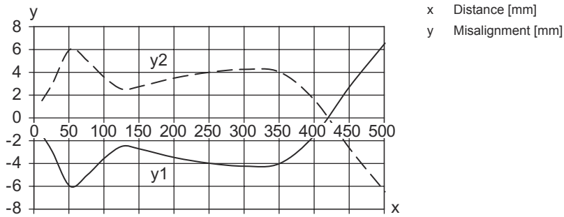
Typ. response behavior (focusing distance 500 mm)
