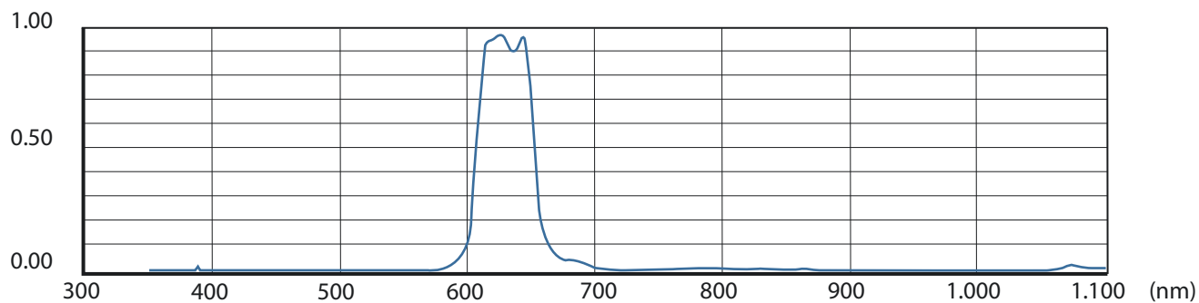
Passband curve
