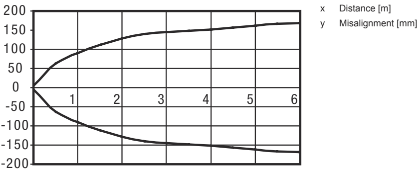
Typ. response behavior (TK 100x100)
