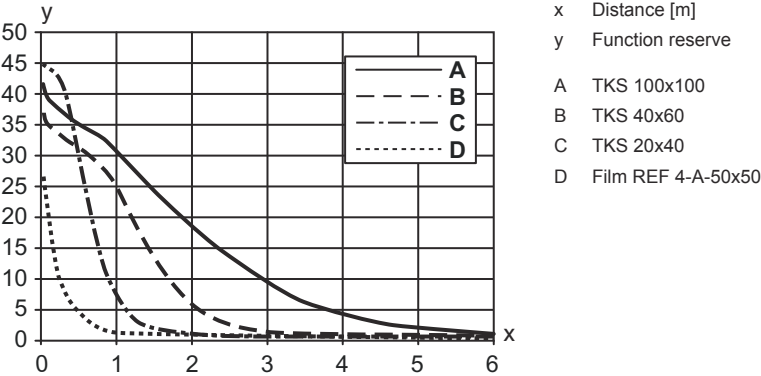
Typ. function reserve
