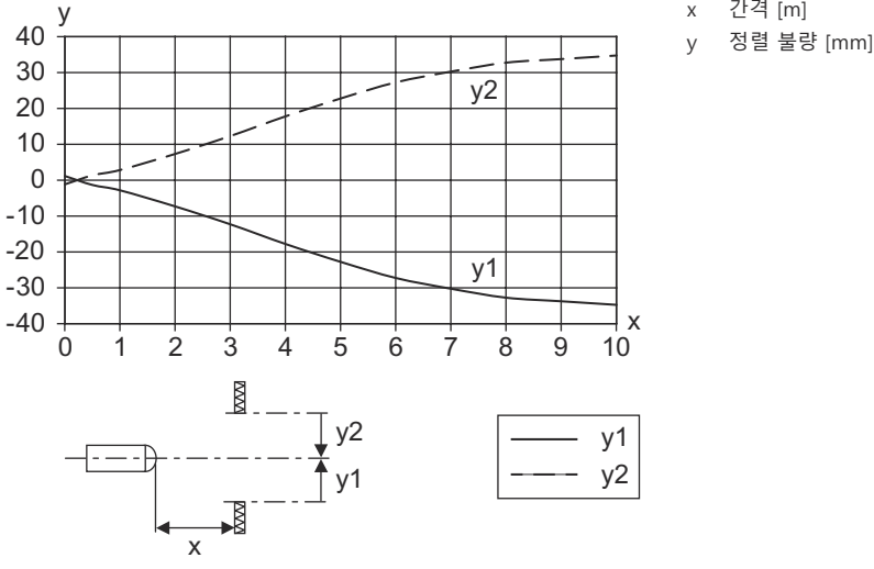
전형적인 반응 거동(TKS100x100)
