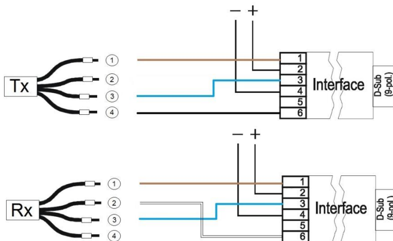
Figura 1: CSL505-Interface
