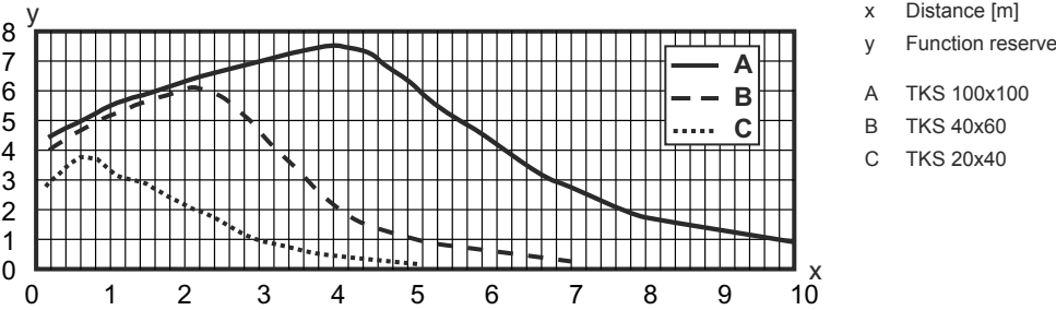
Typ. response behavior (TKS100x100)
