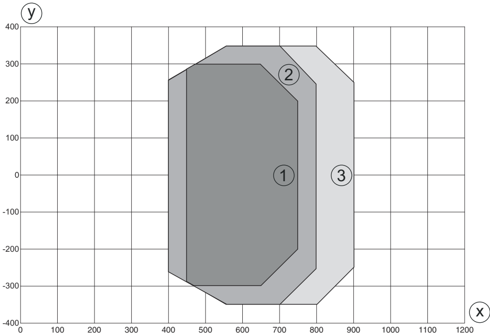
Lesefeldkurve Medium Density
