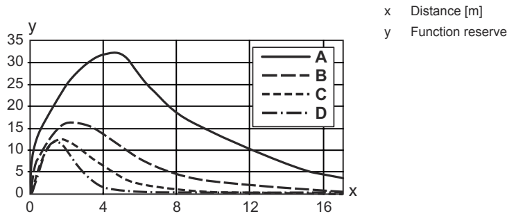
Typ. function reserve
