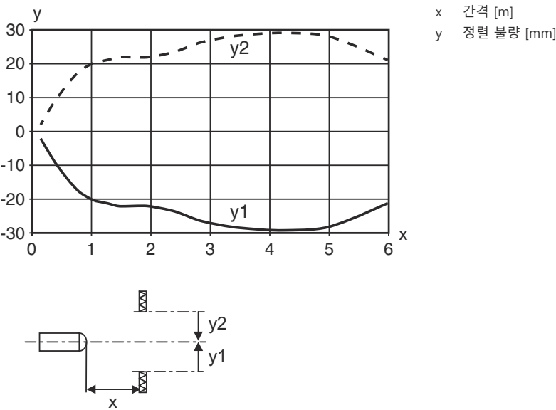
전형적인 반응 거동(TKS100x100)
