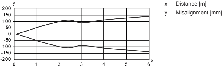
Typ. response behavior (TKS100x100)
