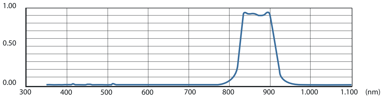
Passband curve
