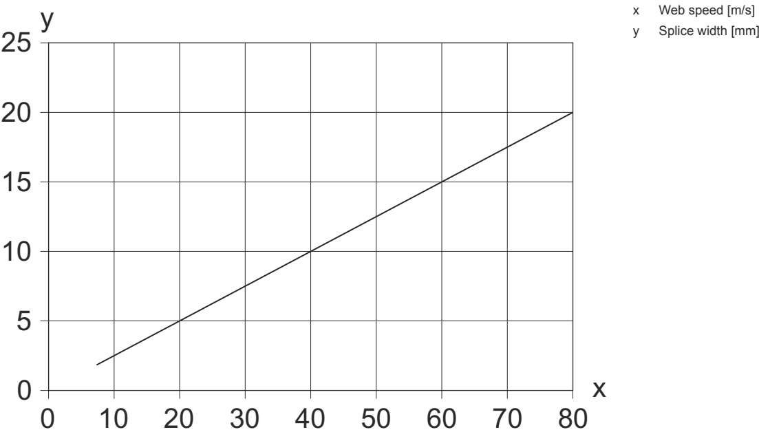
Splice width in dependence of web speed
