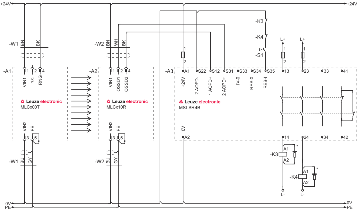
Circuit diagram example with downstream MSI-SR4B safety relay
