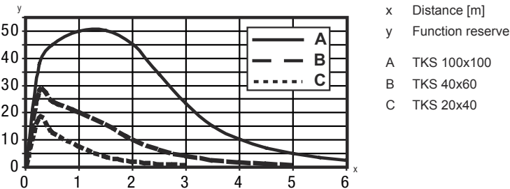
Typ. function reserve (axial model)
