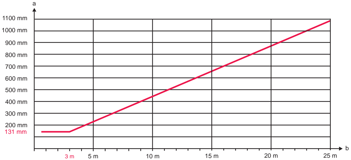
Fig. 5.2: Minimum distance to reflective surfaces depending on protective field width
