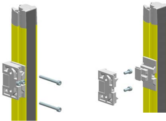
Fig. 5.7: Mounting via swiveling mounting brackets BT-2SB05 and M5 screws
