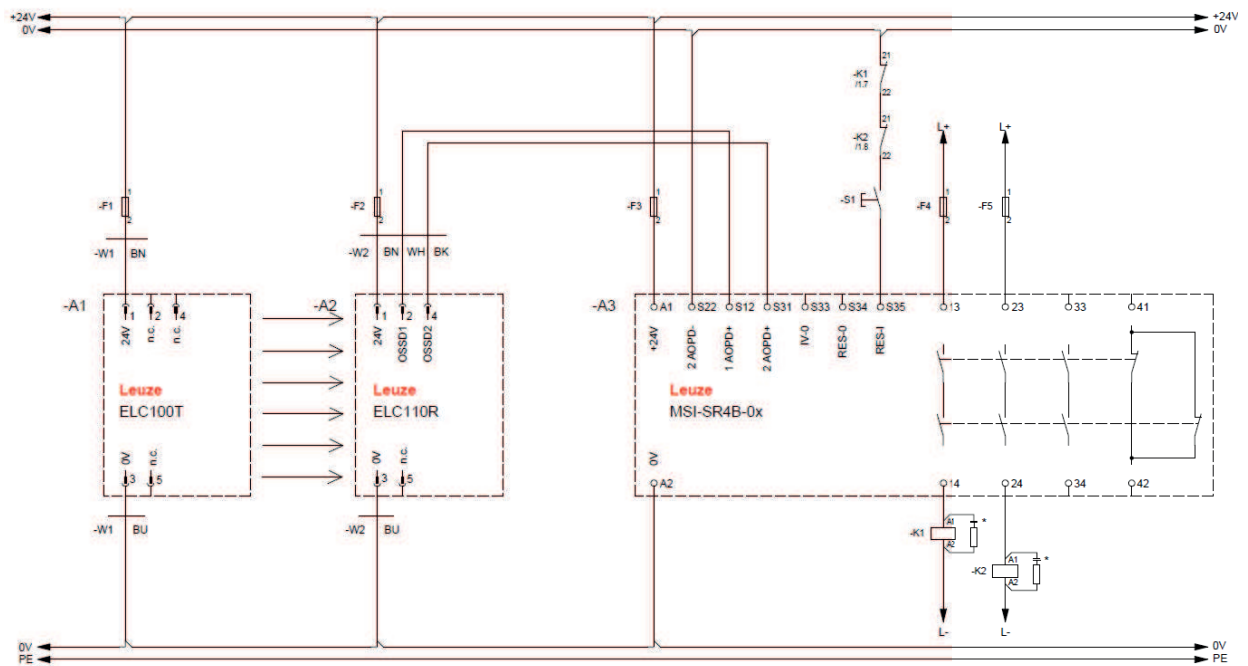
Fig. 6.3: Circuit diagram example with downstream MSI-SR4B safety relay
