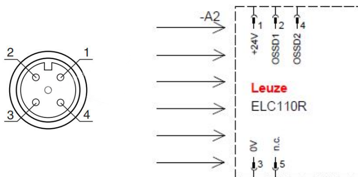
Fig. 6.2: Pin assignment and connection diagram receiver
