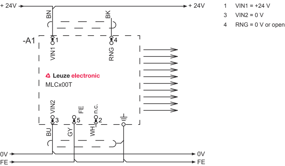
Transmission channel C1, standard range
