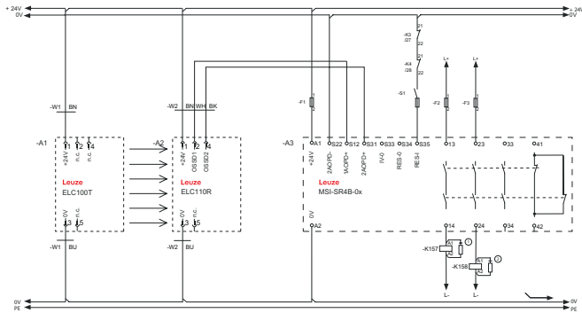
1.2 Spark extinction circuit, suitable spark extinction provided
