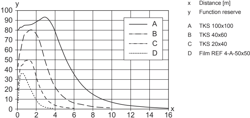
Typ. function reserve
