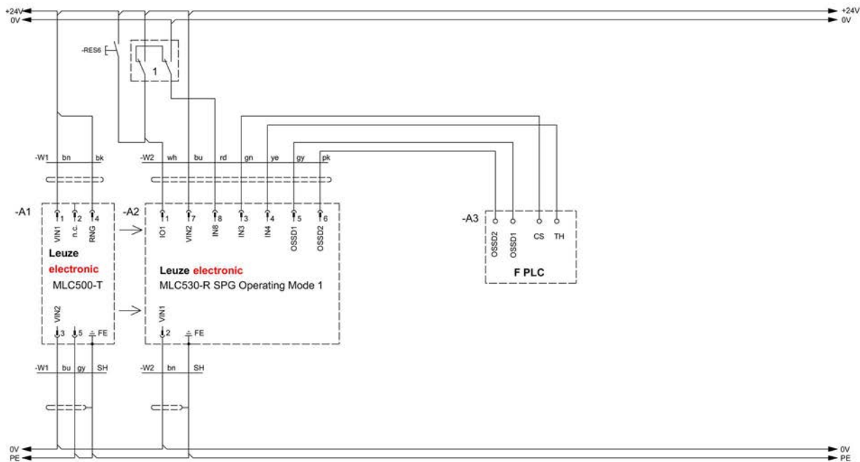
Fig. 8.4: Operating mode 1: connection example with Smart Process Gating (SPG)
