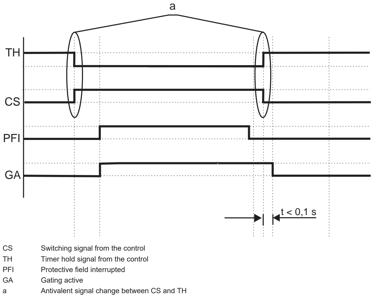
Fig. 4.8: Controlled gating end in operating modes 1 and 6
