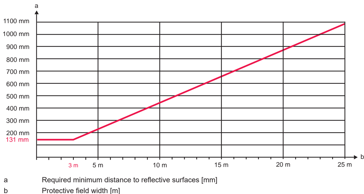
Fig. 6.3: Minimum distance to reflective surfaces as a function of the protective field width
