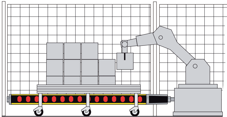
Fig. 4.4: Reduced resolution; several sufficiently small objects can move simultaneously in the protective field or be removed
