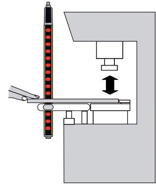
Fig. 4.4: Reduced resolution; several sufficiently small objects can move simultaneously in the protective field or be removed
