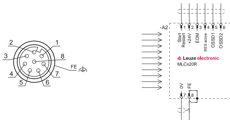
Fig. 7.4: Pin assignment and connection diagram receiver
