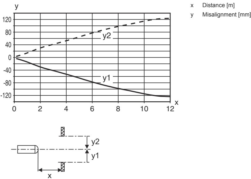
Typ. response behavior (TKS100x100)
