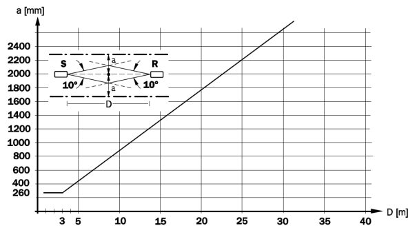
Fig. 4.2: Minimum distance "a" as a function of distance "D" for testable single-beam safety light barriers with 10° aperture angle
