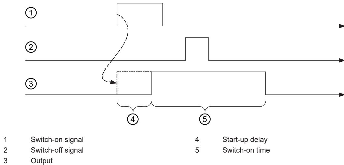
Fig. 8.6: Example 2: Start-up delay > 0 and switch-on time > 0
