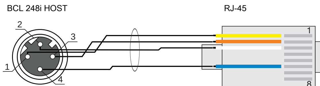
Fig. 6.6: HOST to RJ-45 cable assignments
