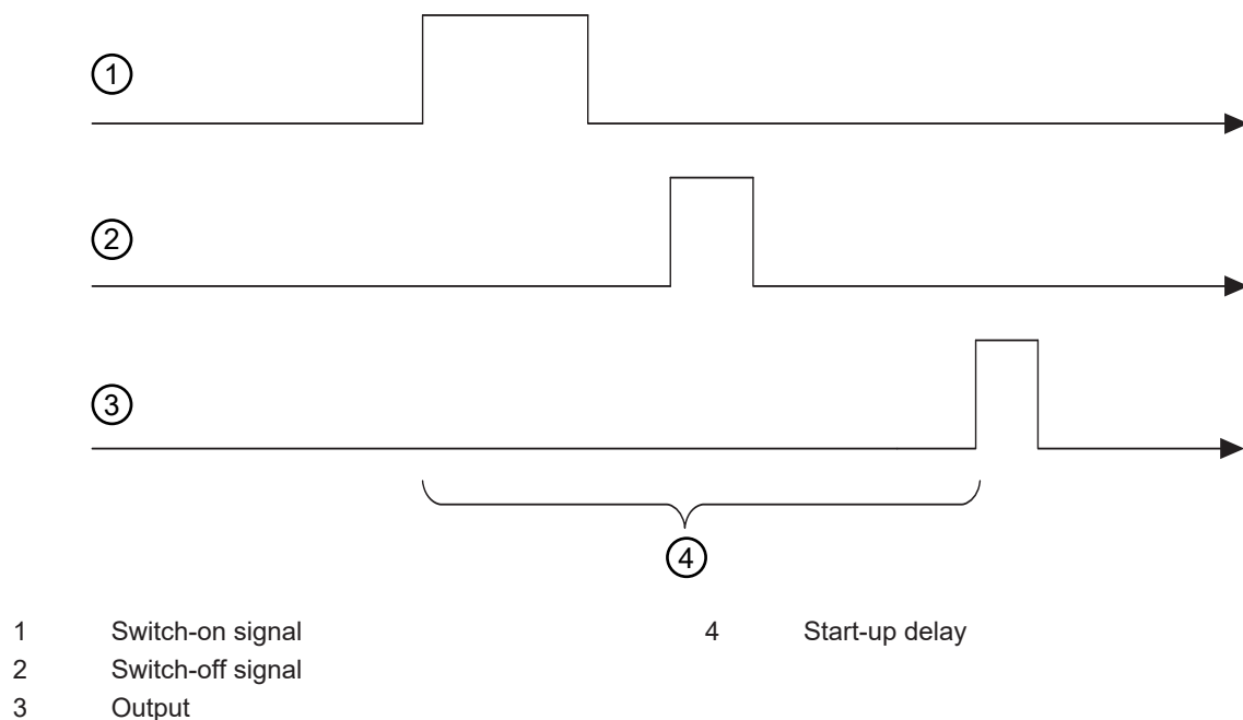
Fig. 8.7: Example 3: Start-up delay > 0 Switch-off signal prior to lapsing of the start-up delay
