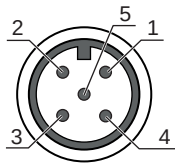
Fig. 6.2: M12 connector, 5-pin, A-coded
