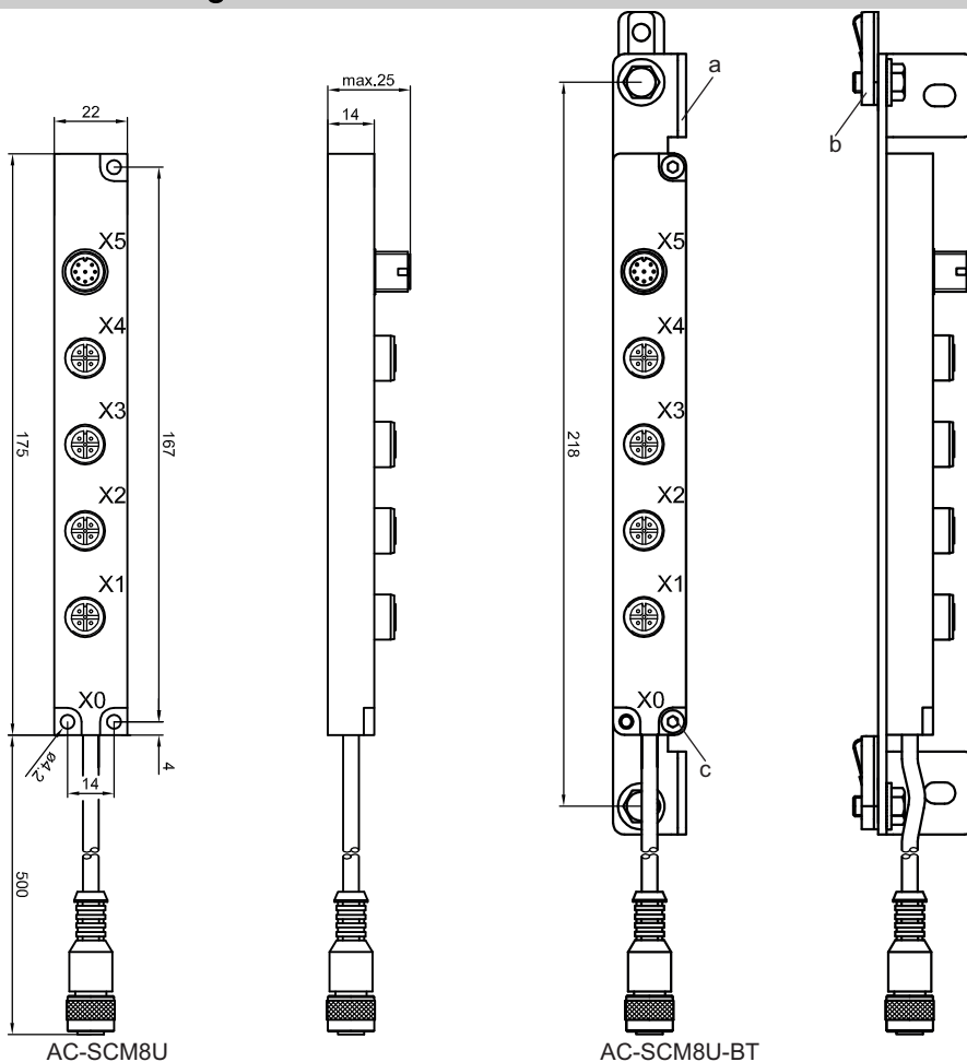
a = Montageplatte b = Nutenstein c = Zylinderschraube M4x16
