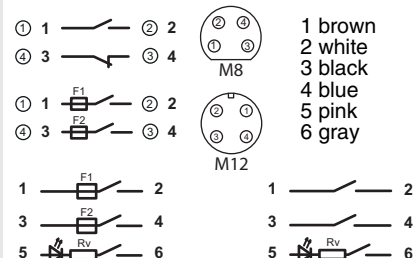
MC3x with wire and pin assignment
